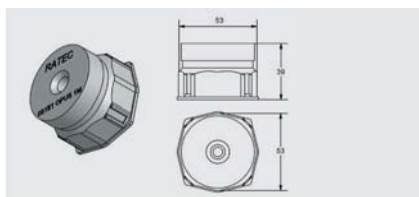
➤ Electrical box magnet for OPUS 1 M
