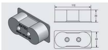
➤ Electrical box magnet for OPUS 2 M
