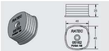
➤ Electrical box magnet for FUGA 1 M
