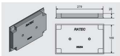
➤ Electrical box magnet for connection box Spelsberg K4
