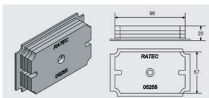
➤ Electrical box magnet for transition box Spelsberg K0
