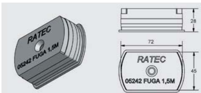
➤ Electrical box magnet for FUGA 1,5 M
