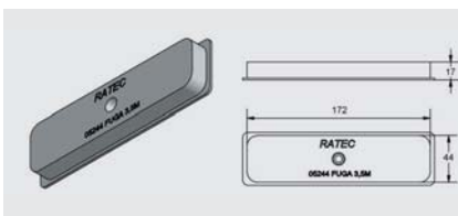
➤ Electrical box magnet for FUGA 3,5 M
