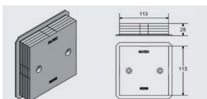
➤ Electrical box magnet for connection box Spelsberg K3
