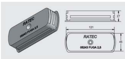
➤ Electrical box magnet for FUGA 2,5 M
